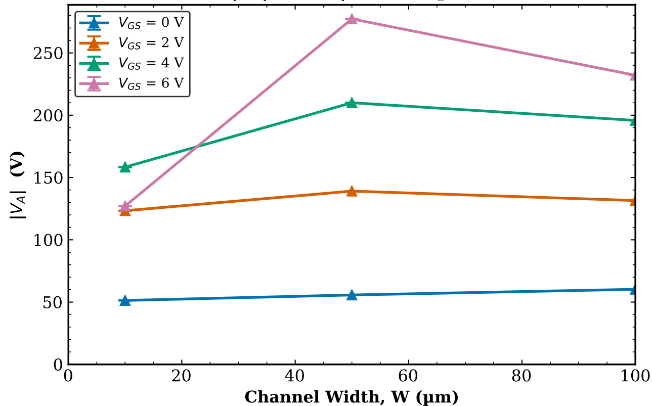
TFT1 Transistor 2 |V_A| vs W | L = 80\text{ }\mu\text{m}
